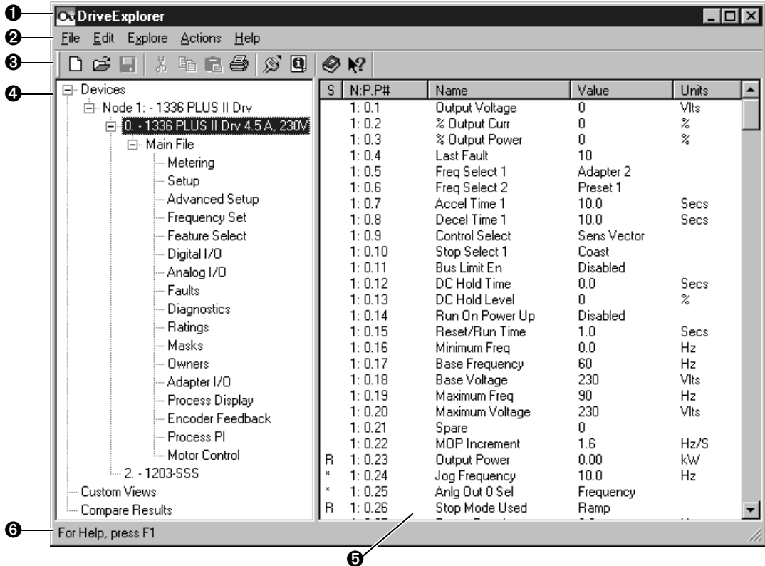
Figure 1.6 DriveExplorer Window
