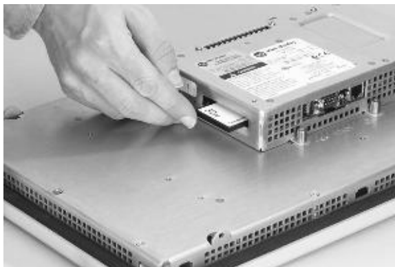
CompactFlash Card Slot on PanelView Plus 700 and 1500 terminals that support FactoryTalk View Machine Edition software version 5.1 or earlier.
