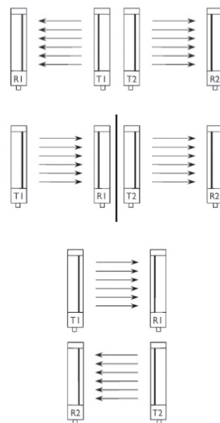
Figure 11 - Multiple GuardShield Micro 400 Safety Light Curtain Alignment Options
