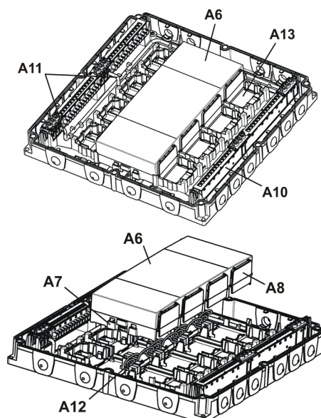
figure 3: Mounting / Dismounting the SELV (class 2) cover
