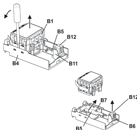
figure 7: Dismounting of a RS module
