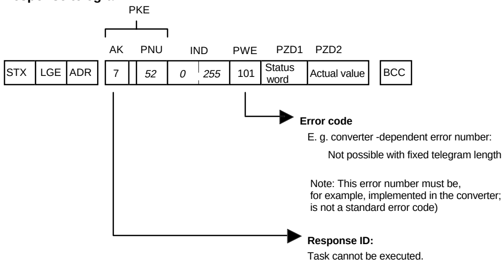
Fig. 8.3: Telegram structure to example 3
