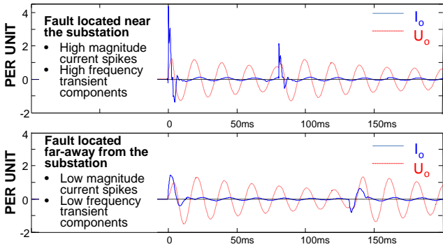
Figure 1: Damping of fault transients due to fault location.
