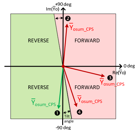
Figure 3: Behaviour of the directional phasor in relation to the operation characteristics of the novel method.
