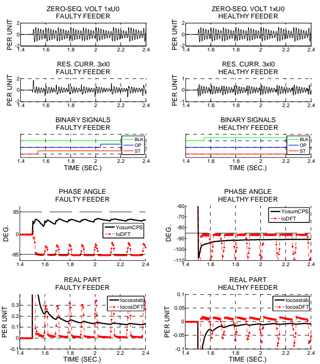
Figure 6: Restriking earth fault with damped transients.
