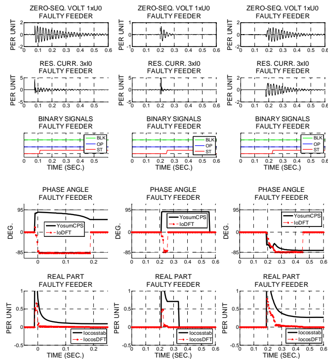
Figure 7: Three examples of temporary earth faults located in the protected feeder.
