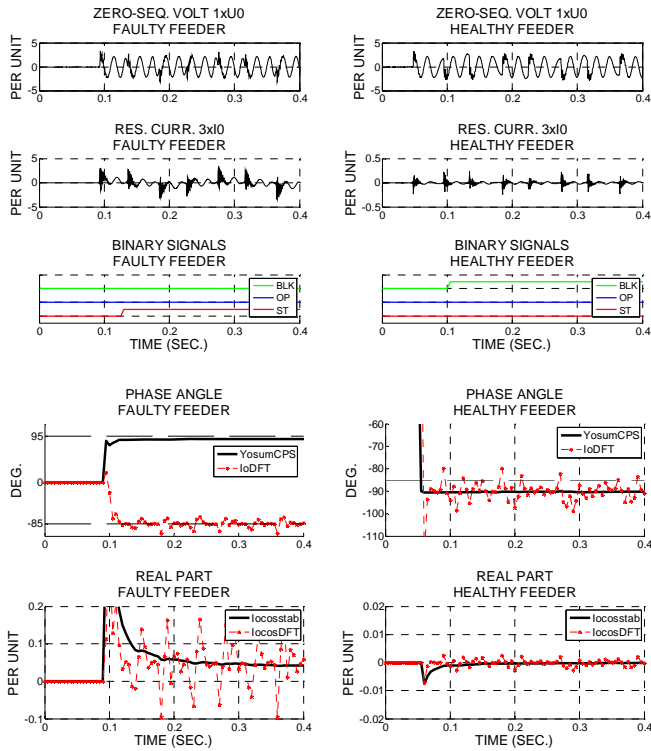
Figure 5: Restriking earth fault with high frequency components.
