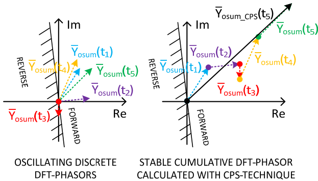
Figure 2: Illustration of the cumulative phasor summing concept (faulted feeder).
