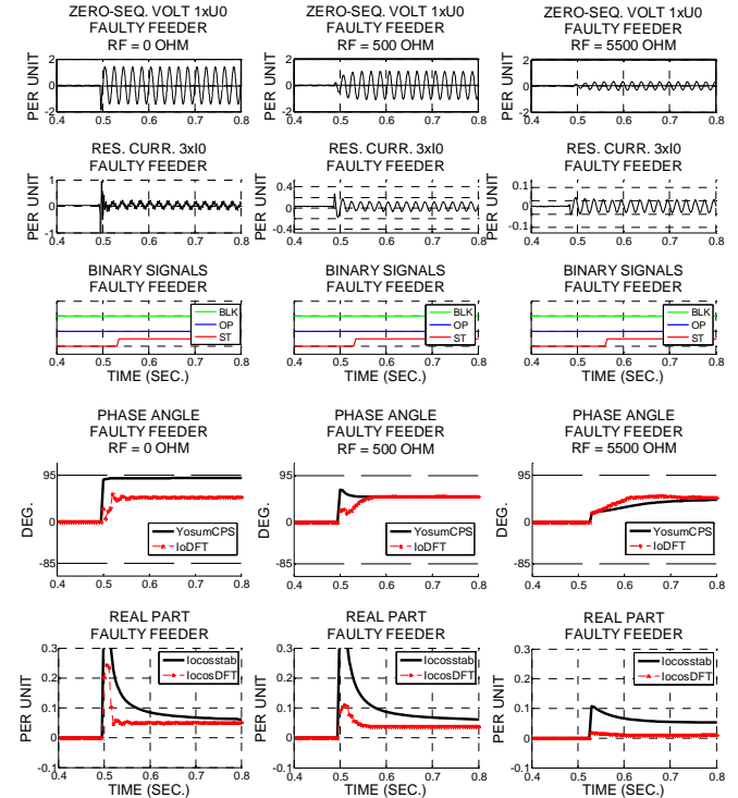
Figure 8: Permanent earth fault with fault resistance of 0, 500 and 5500 ohm.
