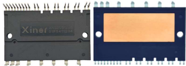
DIP29 DBC (52.5*31*5.6mm)
