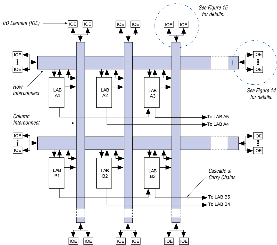
Figure 12. Interconnect Resources
