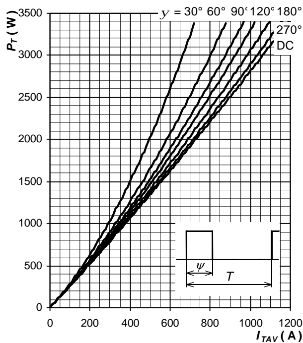
Fig. 9 On-state power loss vs. average on-state current, square waveform, f = 50 \text{ Hz} , T = 1/f
